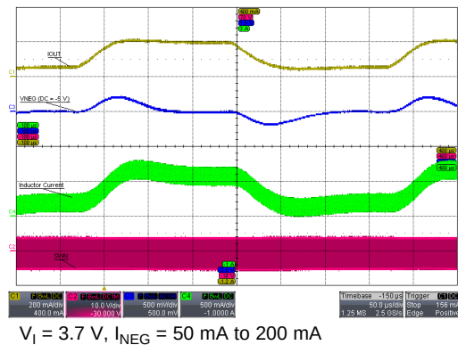
Figure 25. V_{NEG} Load Transient
