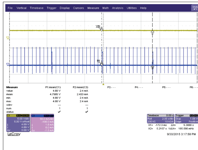
Figure 8. Standby Power
