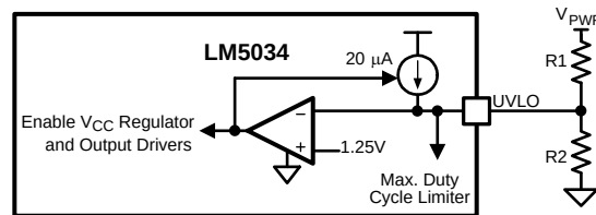
Figure 29. UVLO Circuit
