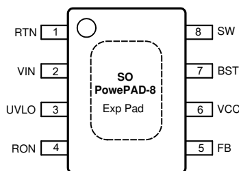
Figure 5-1. 8-Pin HSOP DDA Package Top View
