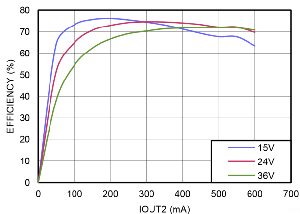
Figure 8-11. Efficiency at 500 kHz, V_{OUT1} = 5\text{ V} , V_{OUT2} = 4.5\text{ V}
