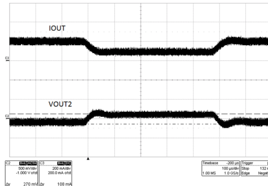
Figure 8-10. Step Load Response ( V_{IN} = 24\text{ V} , I_{OUT1} = 0 , Step Load on I_{OUT2} = 100\text{ mA} to 200\text{ mA} )
