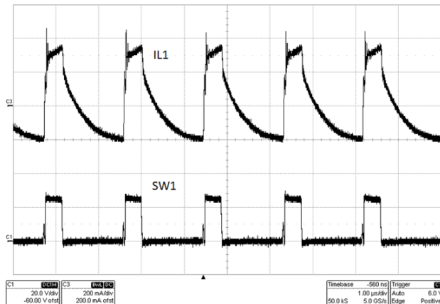
Figure 8-9. Steady State Waveform ( V_{IN} = 24\text{ V} , I_{OUT1} = 100\text{ mA} , I_{OUT2} = 200\text{ mA} )
