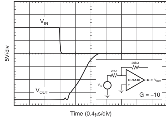
Figure 6-24. Negative Overload Recovery
