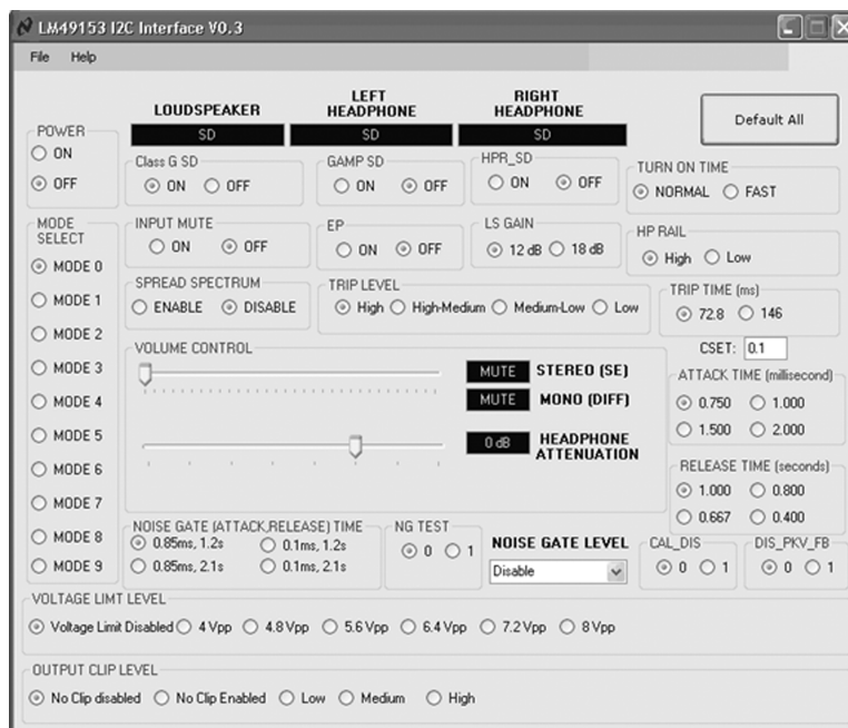
Figure 27. GUI Software
