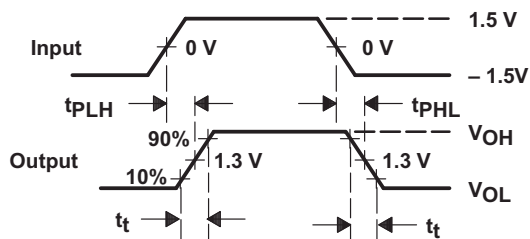
VOLTAGE WAVEFORMS
