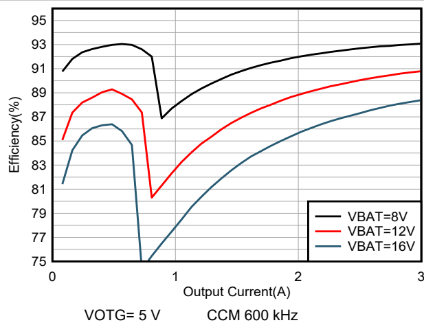
Figure 6-11. OTG Efficiency
