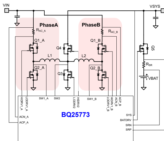
Application Diagram
