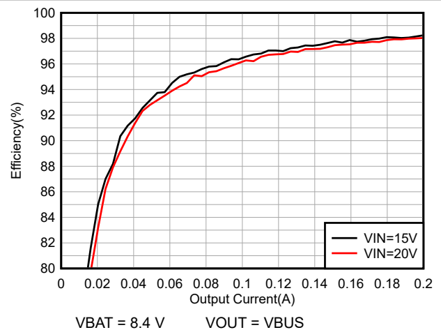
Figure 6-12. PTM Mode Ligh Load System Efficiency
