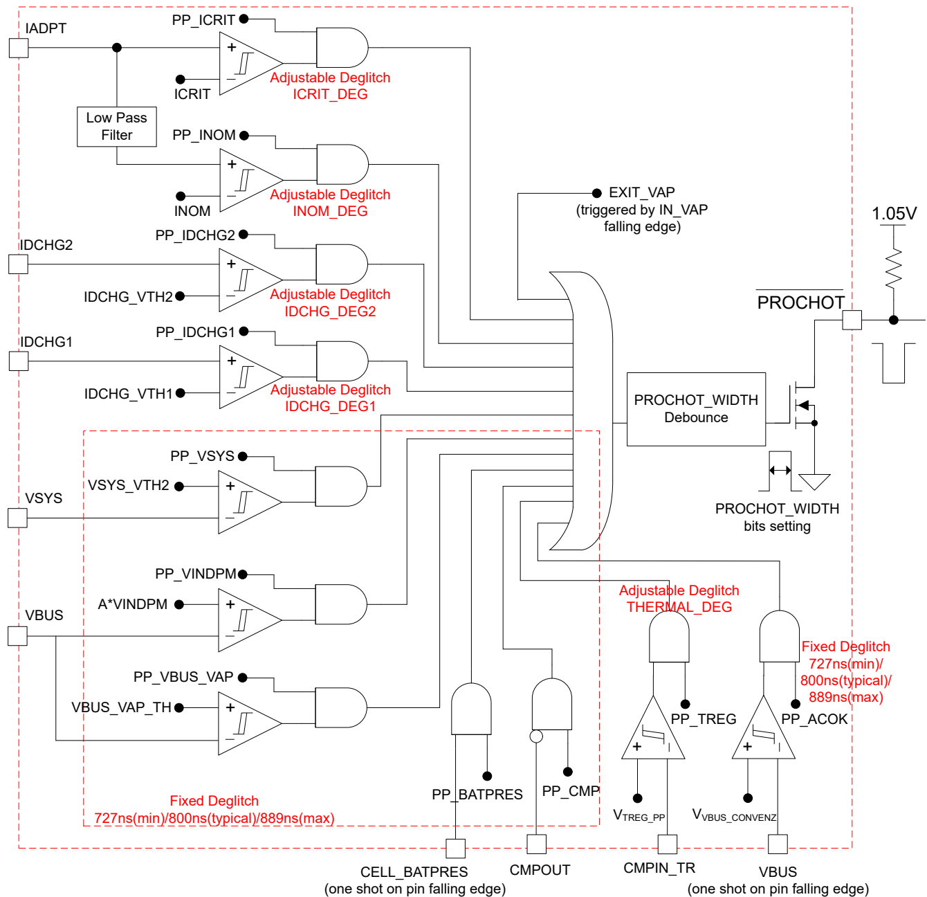
Figure 7-10. PROCHOT Profile
