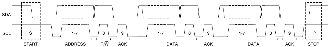
Figure 7-17. Complete Data Transfer
