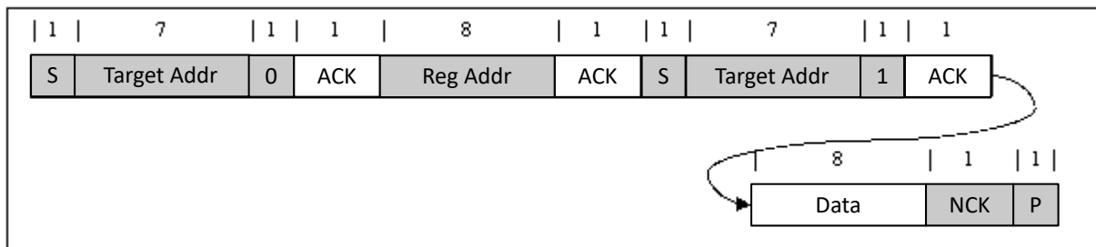
Figure 7-19. Single Read
