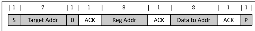
Figure 7-18. Single Write
