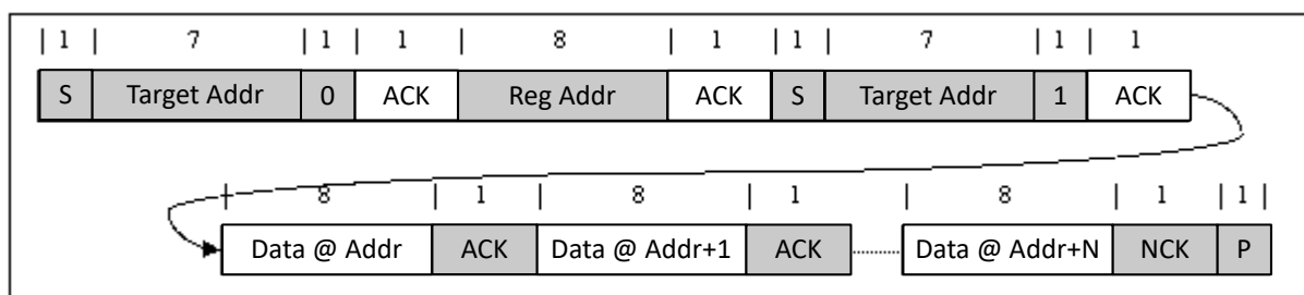
Figure 7-21. Multi Read
