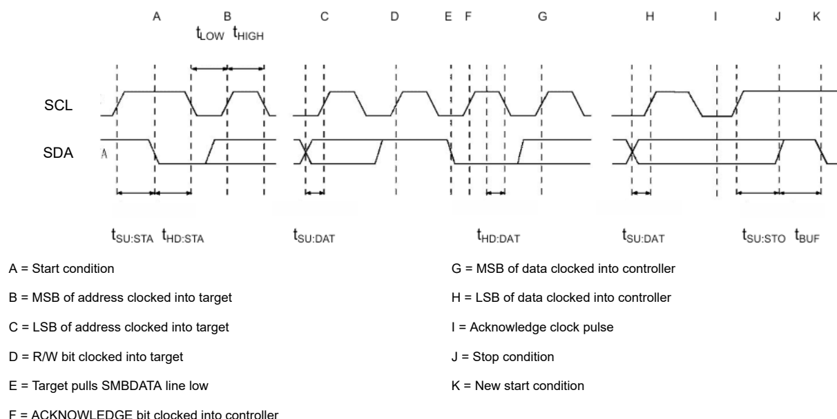
Figure 7-13. I2C Read Timing
