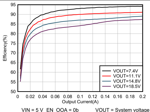
Figure 6-6. Light Load System Efficiency
