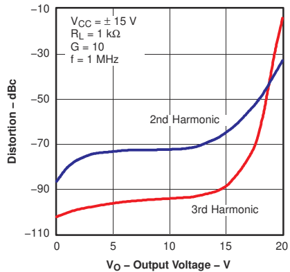
Figure 5-34. Distortion vs Output Voltage
