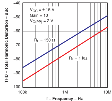
Figure 5-33. Total Harmonic Distortion vs Frequency
