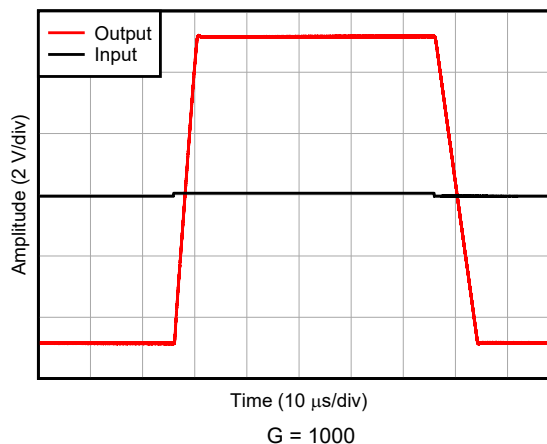
Figure 6-24. Large-Signal Step Response
