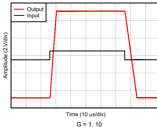
Figure 6-22. Large-Signal Step Response
