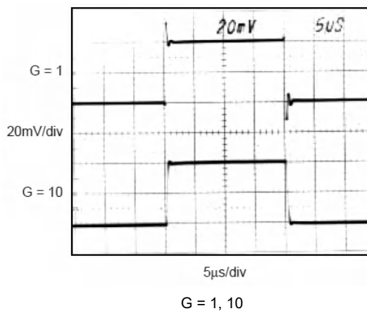
Figure 6-20. Small-Signal Step Response
