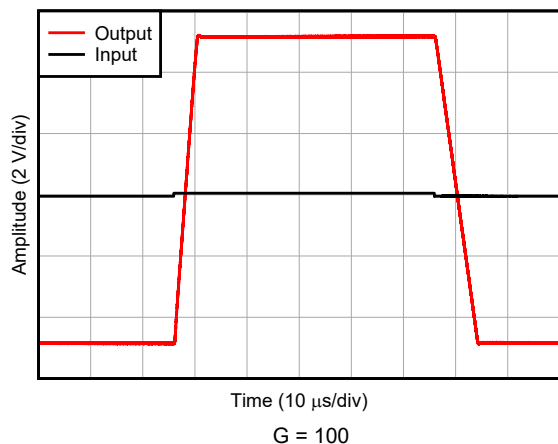
Figure 6-23. Large-Signal Step Response
