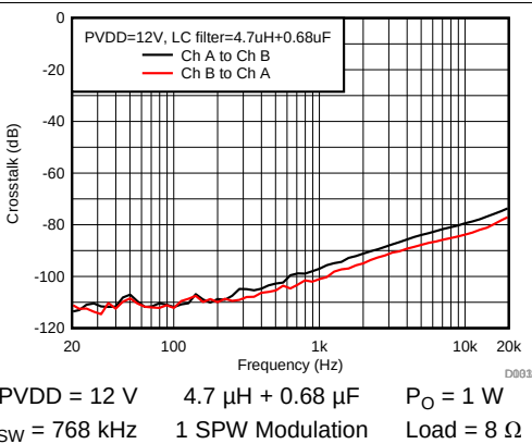
Figure 29. Crosstalk
