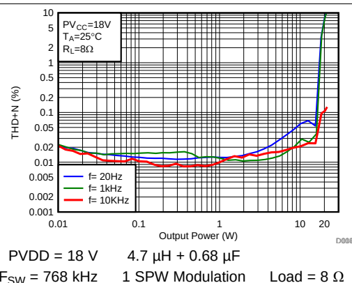
Figure 119. THD+N vs Output Power
