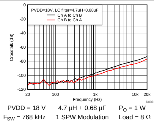
Figure 30. Crosstalk
