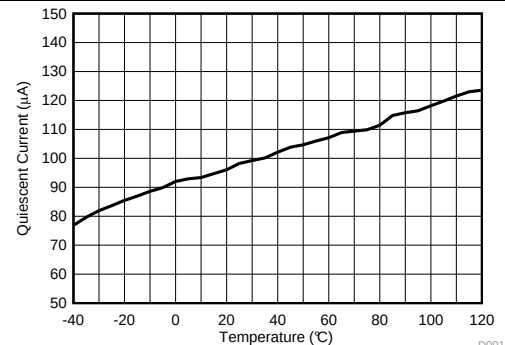
Figure 4. Quiescent Current into VIN vs Temperature
