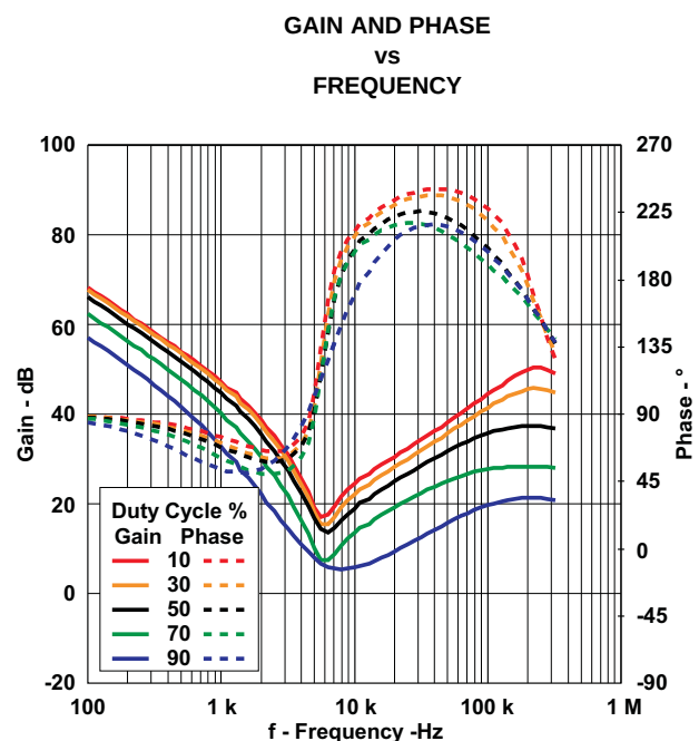
Figure 25. TPS54386-Q1 at 400-mA Peak-to-Peak Ripple Current
