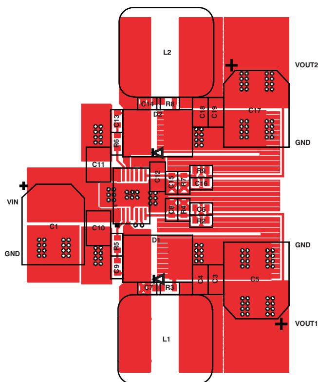
Figure 34. Top Layer Copper Layout and Component Placement
