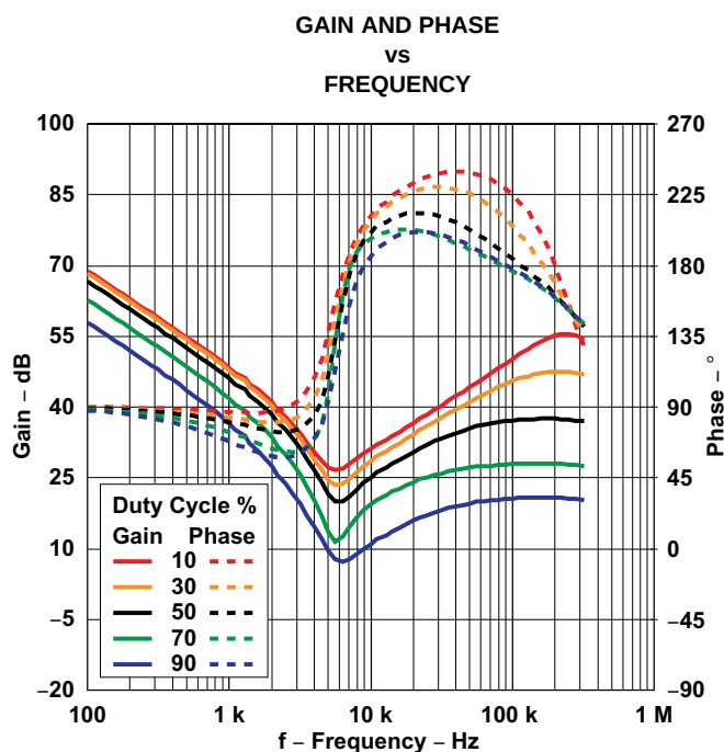
Figure 24. TPS54386-Q1 at 200-mA Peak-to-Peak Ripple Current
