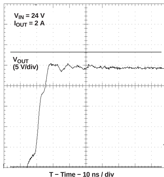
Figure 45. Switch Node Ringing With Snubber and Boost Resistor
