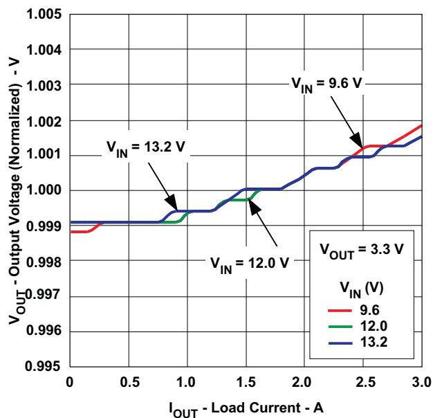
Figure 41. 3.3-V Output Voltage vs Load Current
