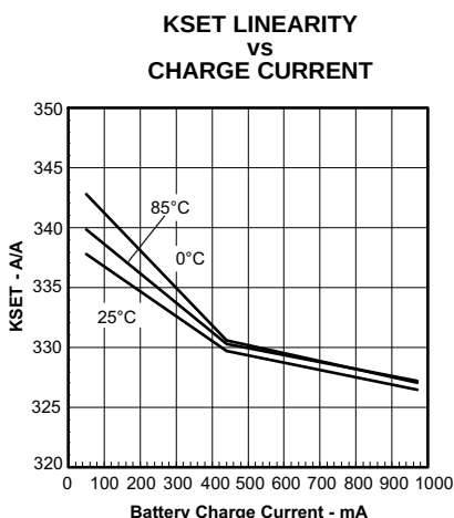
Figure 10. 3.0 < V_{(BAT)} < 4.0 V
