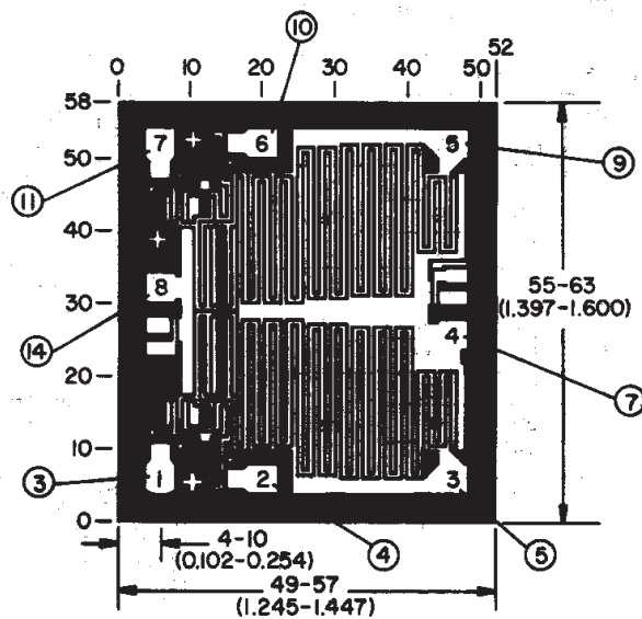
Dimensions and Pad Layout for CD40107BH.
