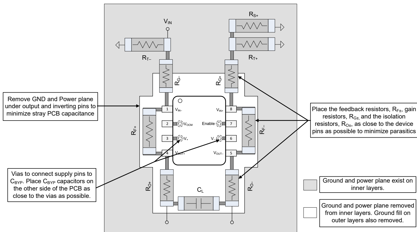
Figure 8-8. Example Layout
