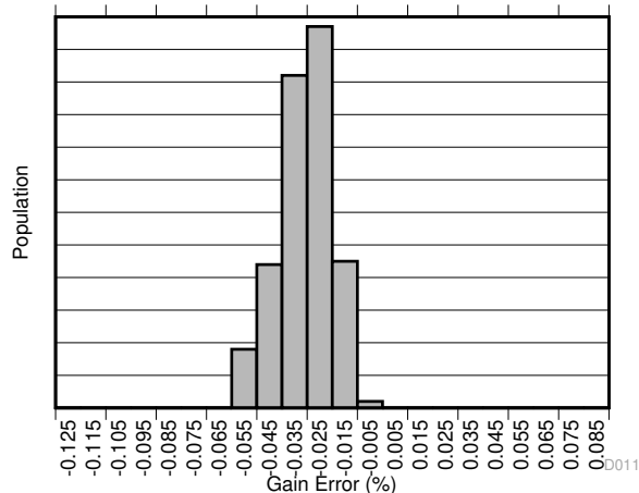
Figure 7-11. Gain Error Production Distribution A1
