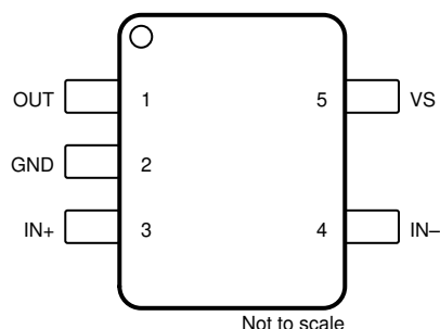
Figure 6-1. INA180-Q1: DBV Package 5-Pin SOT-23 (Pinout A) Top View Figure 6-2. INA180-Q1: DBV Package 5-Pin SOT-23 (Pinout B) Top View
