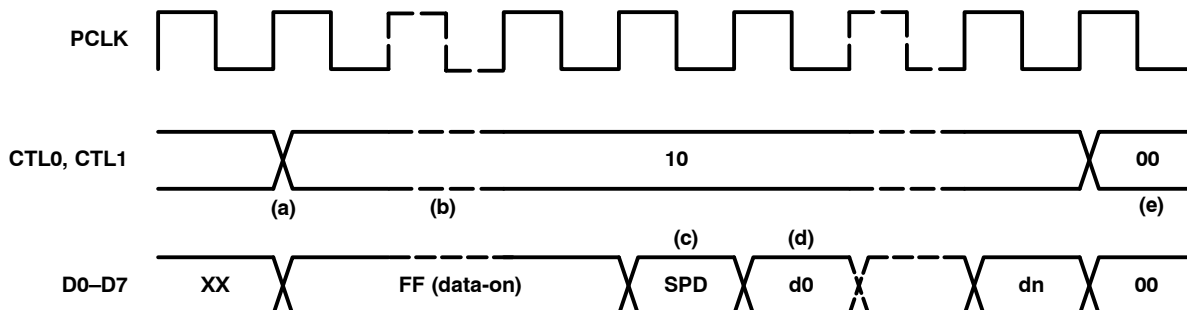
Figure 26. Normal Packet Reception Timing
