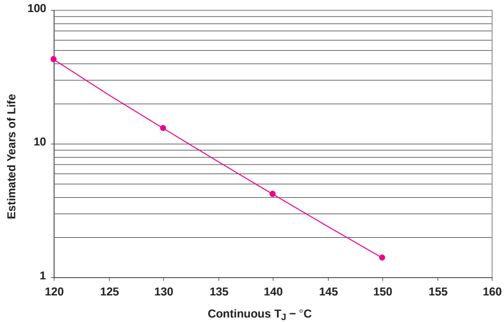
Figure 2. TPS5120 Wirebond Life
