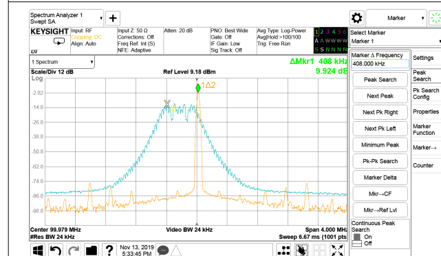
Figure 9-6. 100 MHz With - 0.5% Down Spread With and Without Trace
