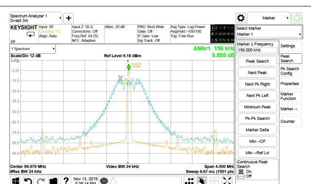
Figure 9-5. 100 MHz With +/- 0.25% Center Spread With and Without Trace
