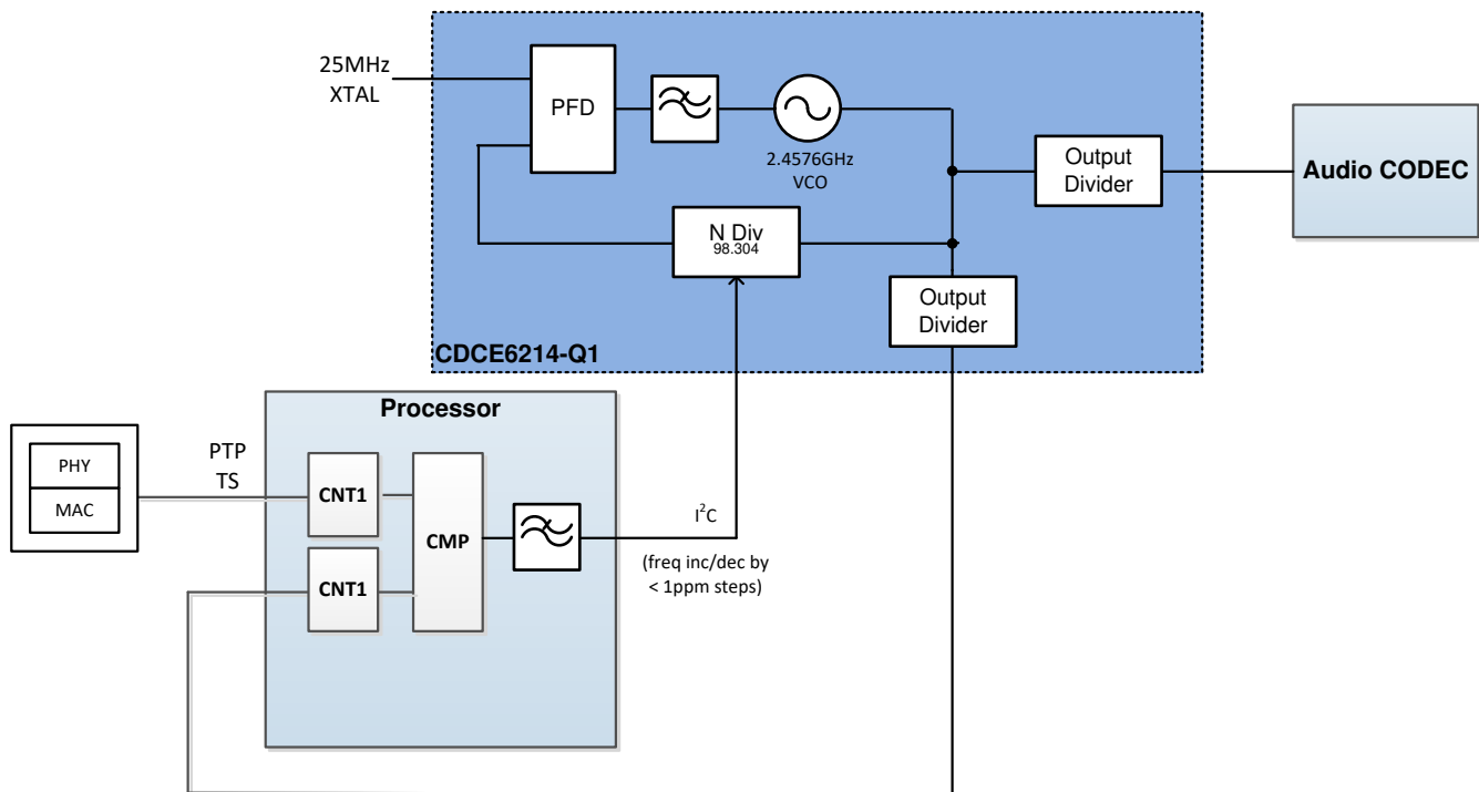
Figure 10-2. eAVB System Block Diagram Using CDCE6214-Q1
