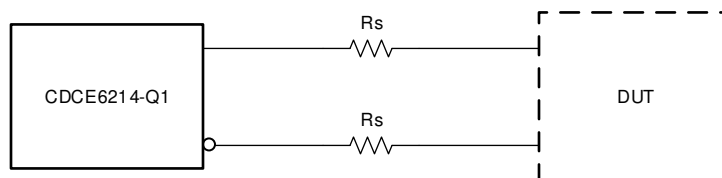
Figure 8-14. LP-HCSL Output
