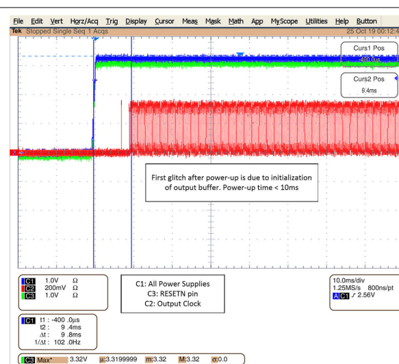
Figure 7-6. All Power Supply = 3.3 V, VDD Ramp Time = 1 ms
