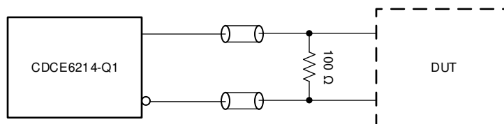
Figure 8-12. LVDS Output - DC-Coupled. Place 100Ω close to the DUT
