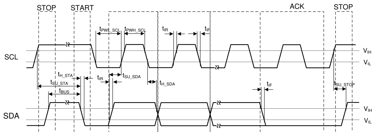
Figure 8-7. I²C Timing
