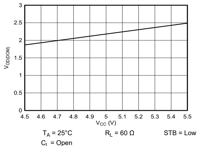
Figure 6-2. V_{OD(DOM)} over V_{CC}
