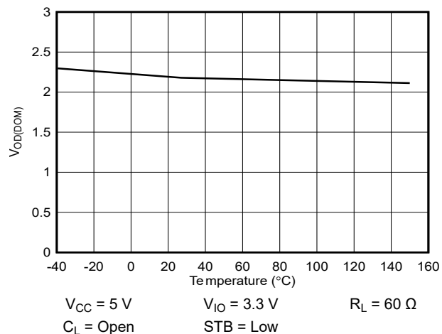
Figure 6-1. V_{OD(DOM)} Overtemperature
