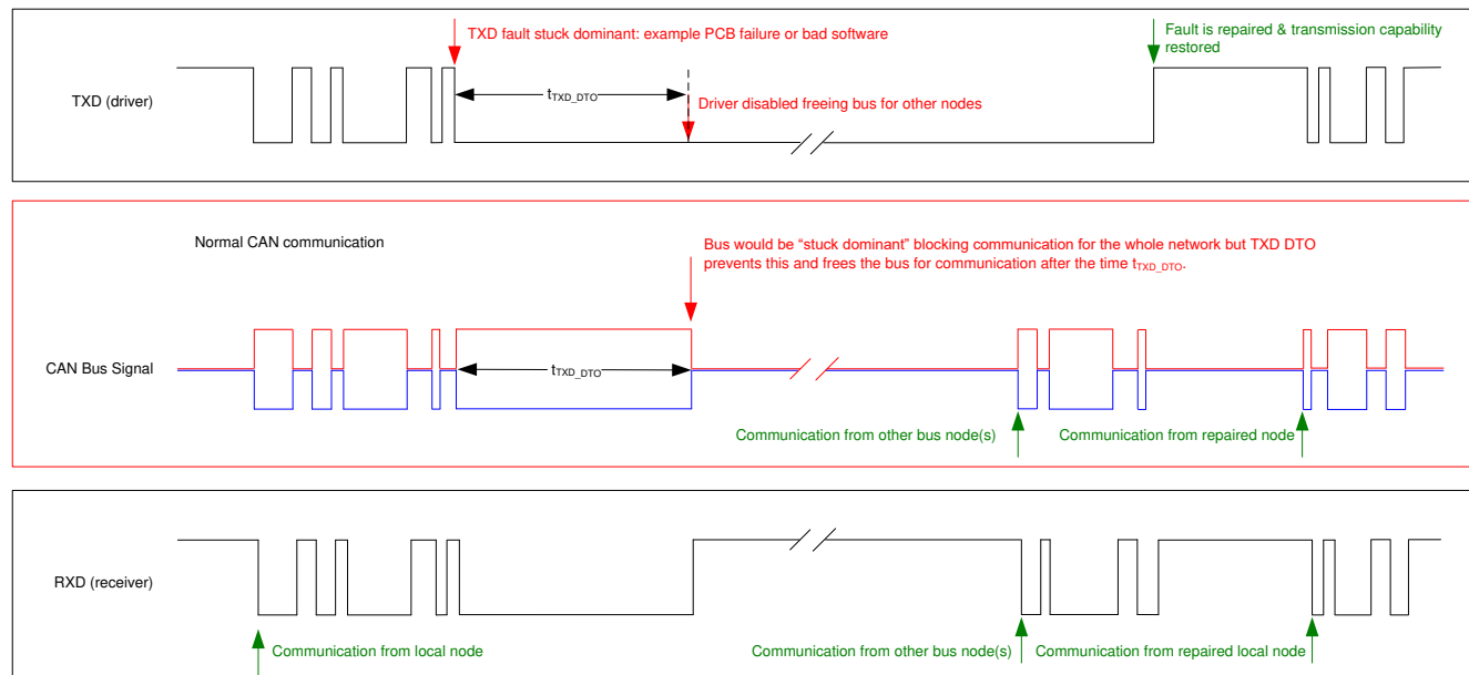
Figure 8-6. Example Timing Diagram for TXD Dominant Timeout
