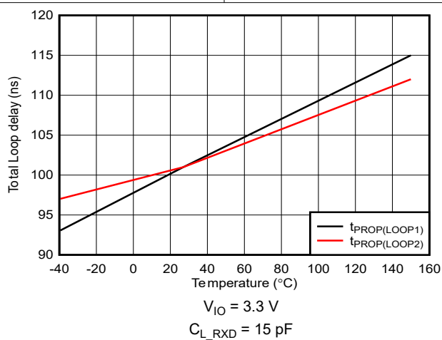
Figure 6-5. Total loop delay t_{PROP(LOOP1)} and t_{PROP(LOOP2)} vs Temperature
