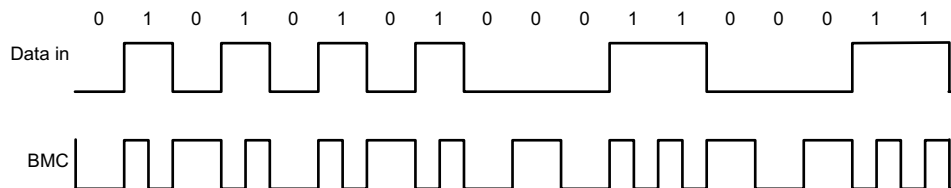
Figure 8-6. Biphas Mark Coding Example
