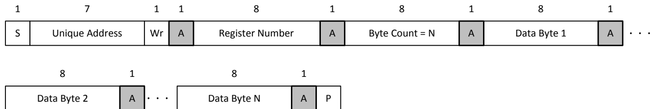
Figure 8-30. I 2 C Unique Address Write Register Protocol
