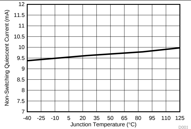
Figure 8. Non-Switching Input Current ( I_{VDD} ) vs. Junction Temperature
