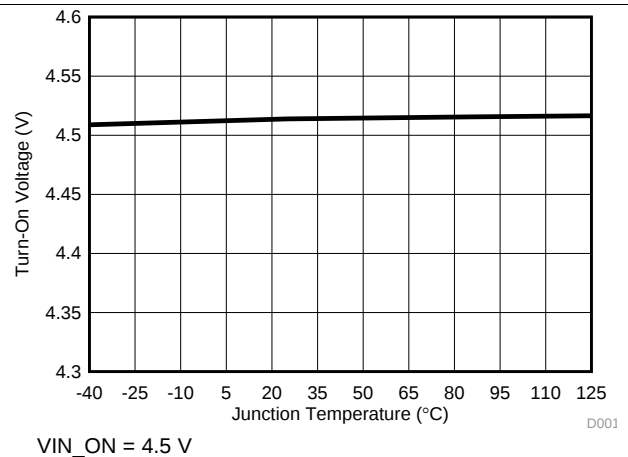
Figure 12. Turn-On Voltage vs. Junction Temperature
