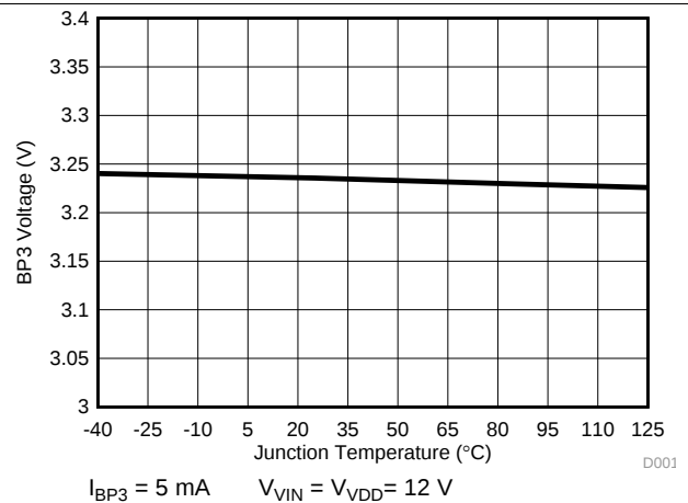
Figure 10. BP3 Voltage vs. Junction Temperature
