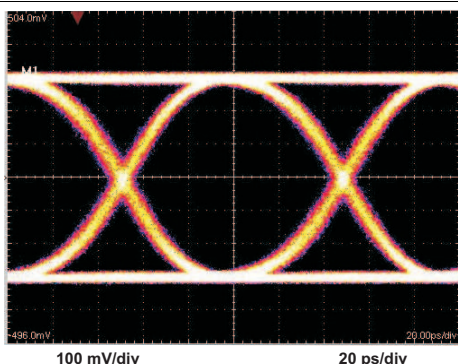
Figure 16. Output Eye-Diagram at 10.3 GBPS vs and Input Voltage (20 mV pp )
