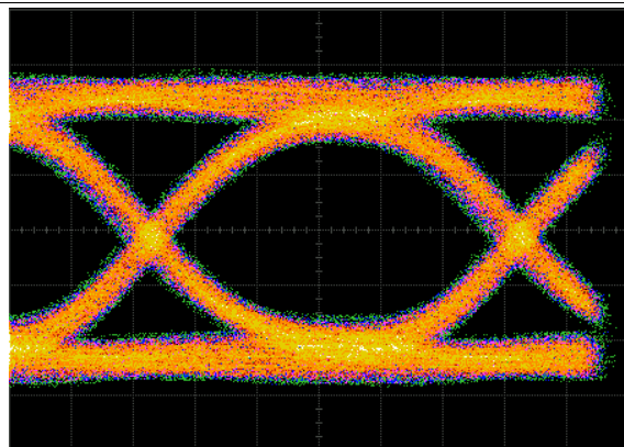
Figure 10. Output Eye-Diagram, 500- \mu\text{A}_{PP} Input Current
