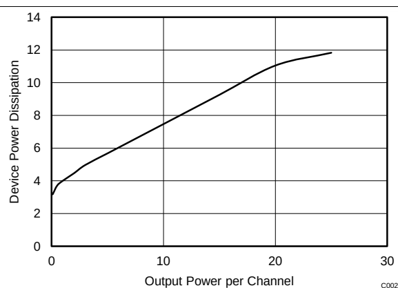
Figure 22. TAS5404-Q1 Device Power Dissipation Four Channels at 4 Ω Each
