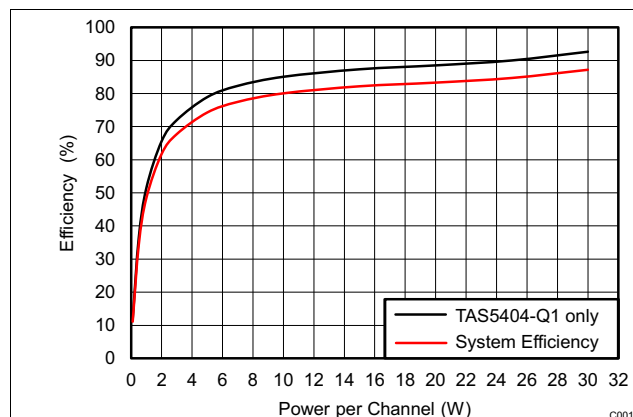
Figure 21. Efficiency Four Channels AT 4 Ω Each
