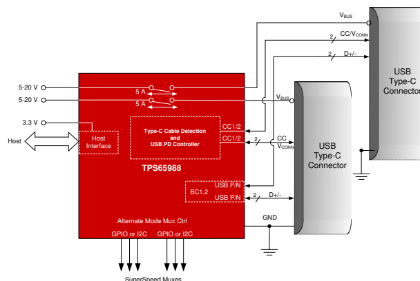
Simplified Schematic
