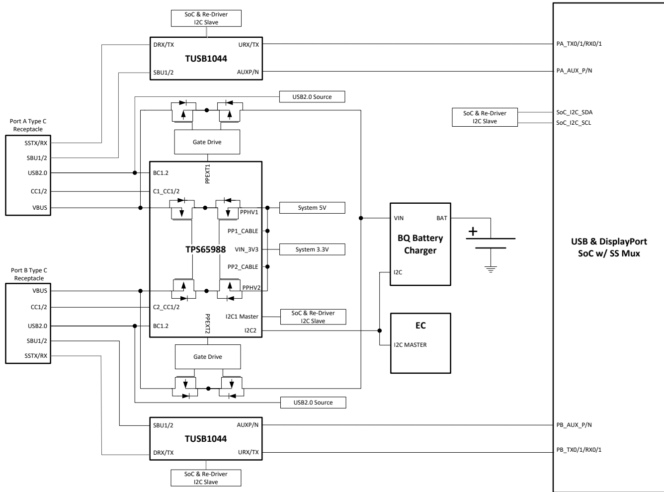
Figure 9-10. TPS65988DJ, SoC and Redriver I2C
