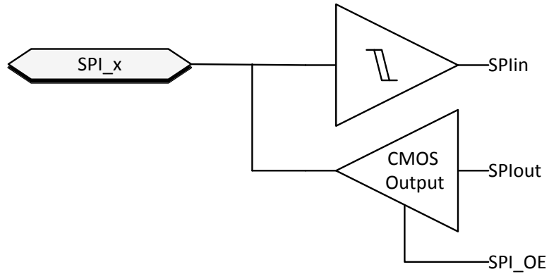
Figure 8-21. SPI Buffer
