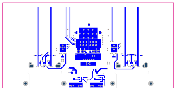
Figure 11-26. SSTXRX2 Layer
