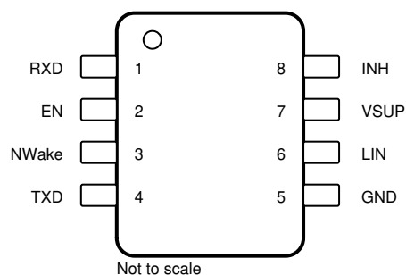
Figure 7-1. D Package, 8-Pin SOIC (Top View)
