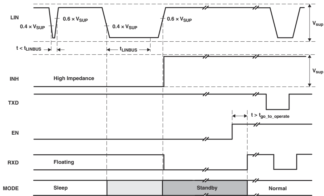
Figure 10-3. Wakeup Through LIN
