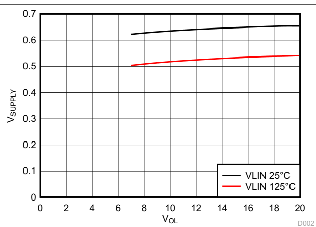
Figure 8-4. V_{OL} vs V_{SUPPLY} and Temperature
