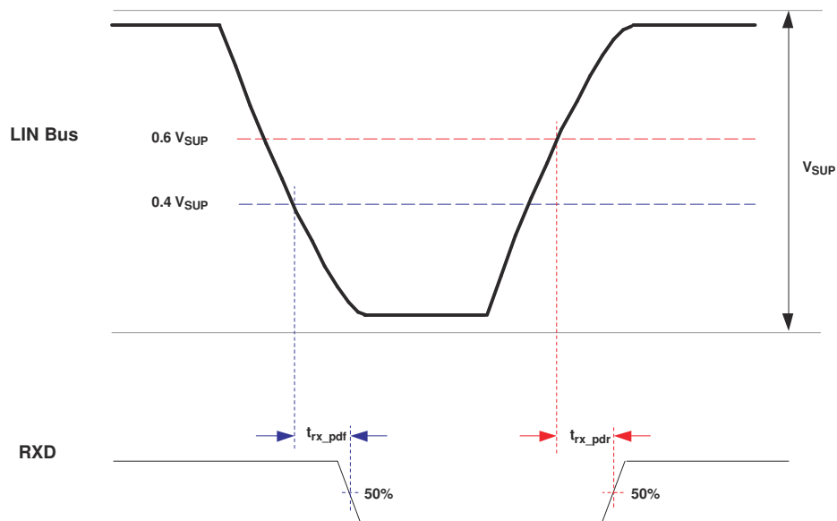
Figure 8-2. Propagation Delay
