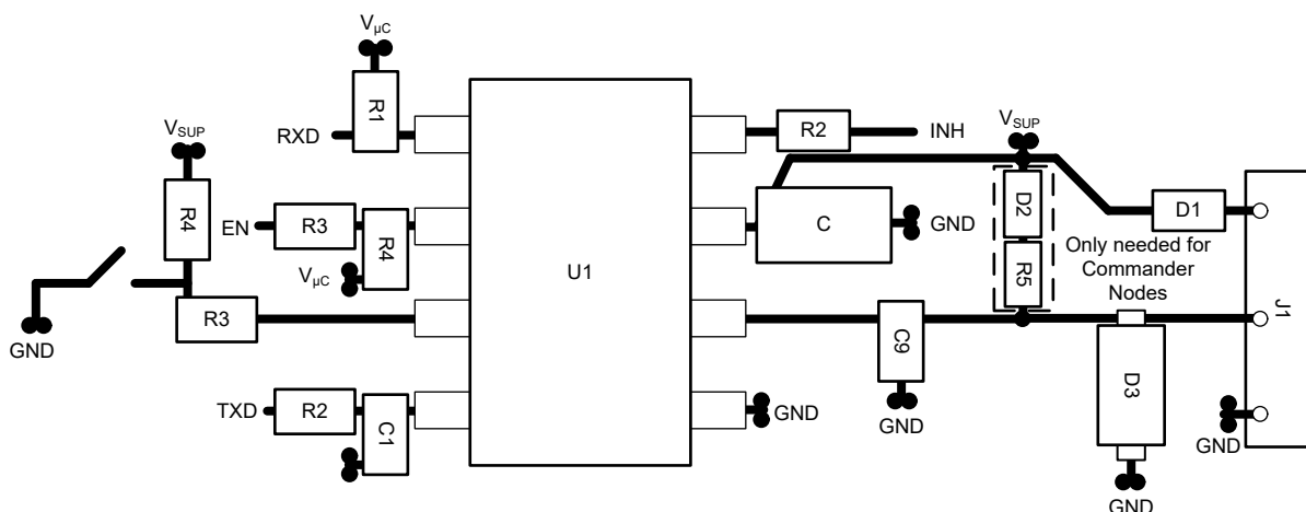
Figure 11-4. TPIC1021A-Q1 Layout
