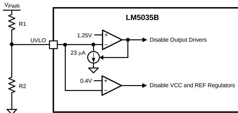
Figure 22. Basic UVLO Configuration
