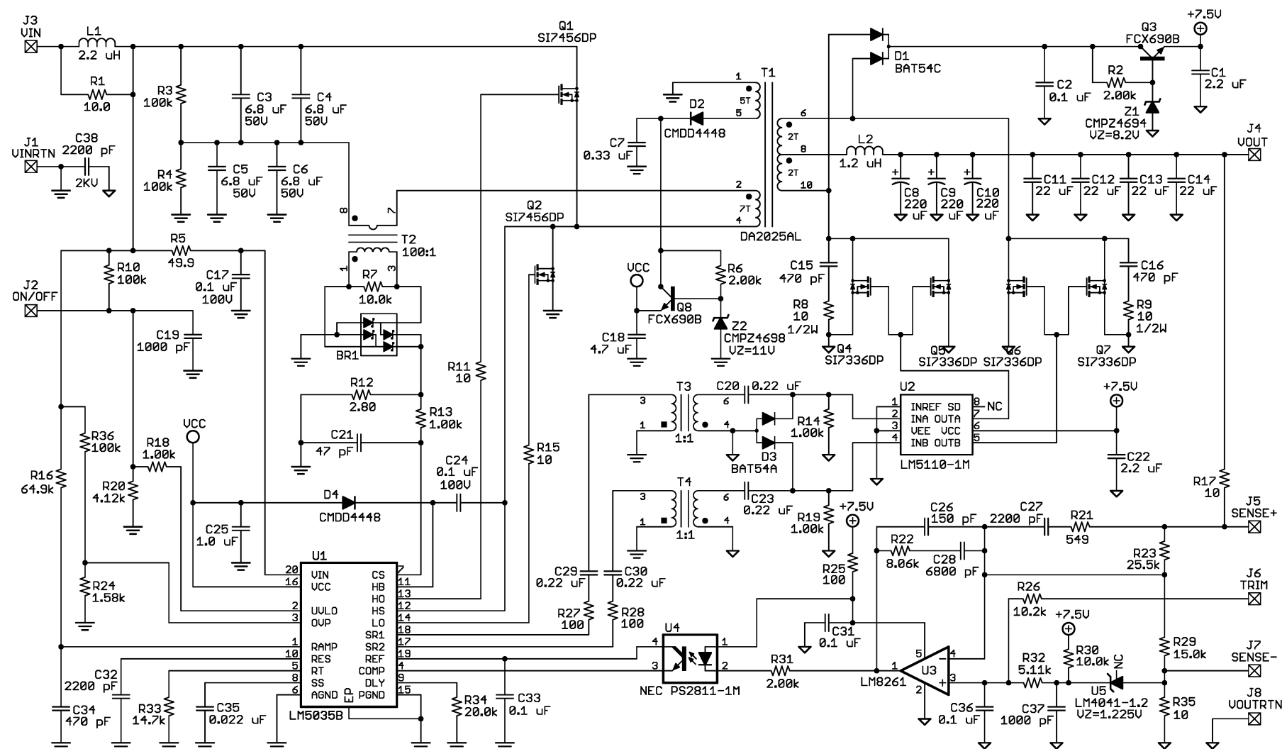
Figure 29. Evaluation Board Schematic
