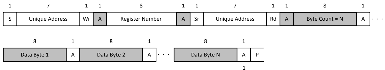
Figure 8-26. I²C Unique Address Read Register Protocol
