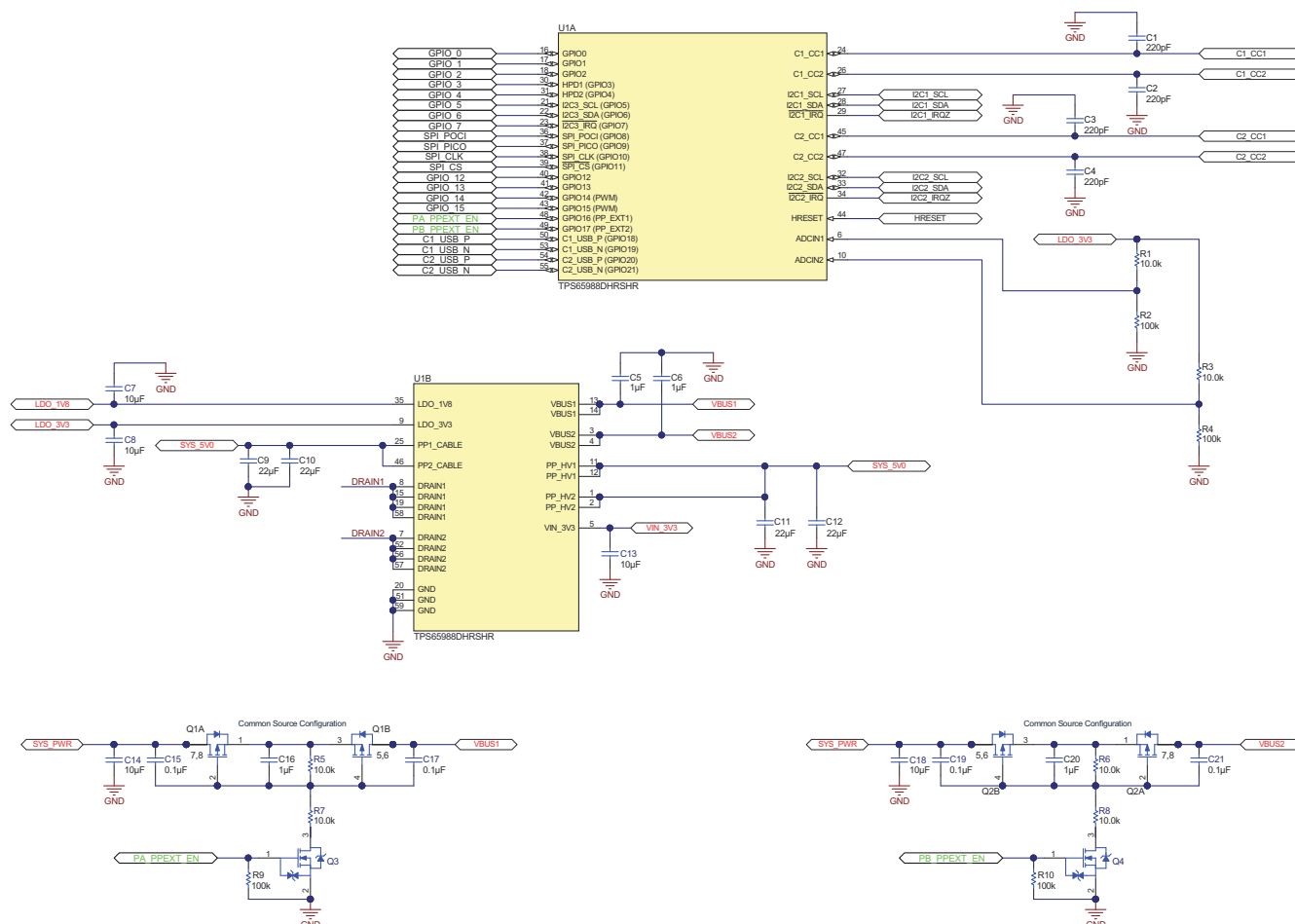
Figure 11-1. Layout Example Device Schematic
