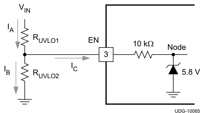
Figure 29. Node Voltage
