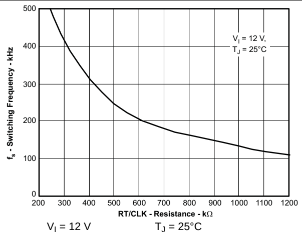
Figure 6. Switching Frequency vs RT/CLK Resistance, Low-Frequency Range
