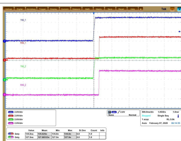
Figure 9-5. t_{\text{PROP(LOOP2)}} Transceiver 1 and Transceiver 2
