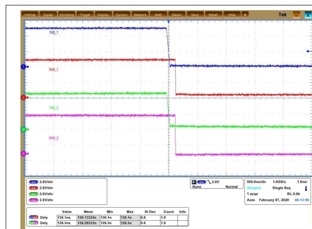
Figure 9-4. t_{\text{PROP(LOOP1)}} Transceiver 1 and Transceiver 2
