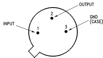
Figure 1. Bottom View See Package NDT0003A
