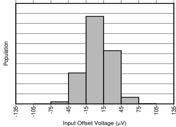
Figure 6-1. INA310A1-Q1 Input Offset Production Distribution
