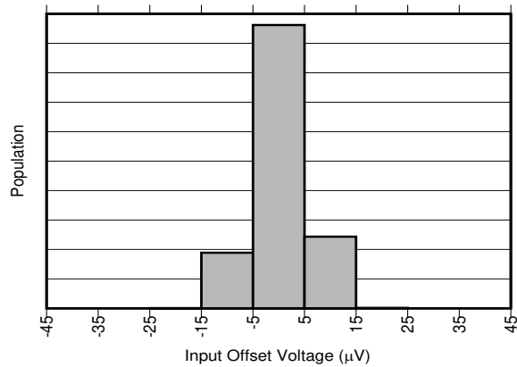
Figure 6-3. INA310A3-Q1 Input Offset Production Distribution
