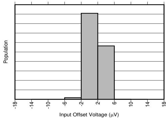
Figure 6-5. INA310A5-Q1 Input Offset Production Distribution
