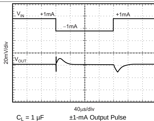
Figure 18. Load Transient
