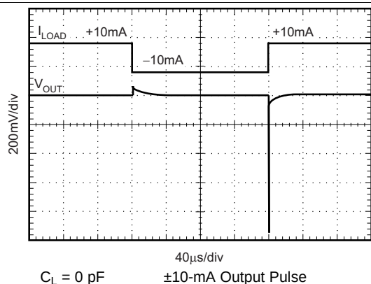
Figure 15. Load Transient
