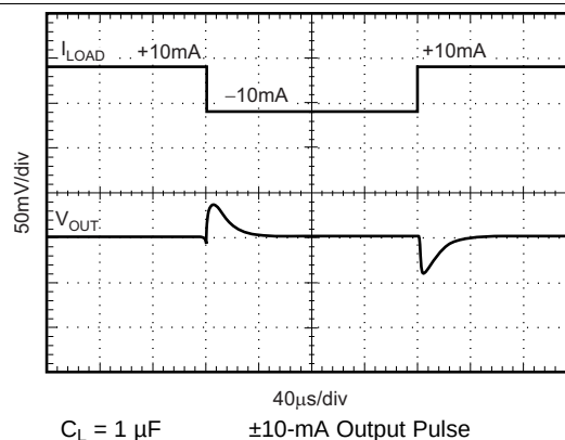
Figure 16. Load Transient
