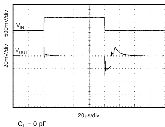
Figure 13. Line Transient
