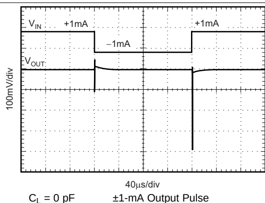
Figure 17. Load Transient
