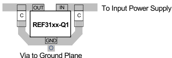
Figure 33. Layout Example
