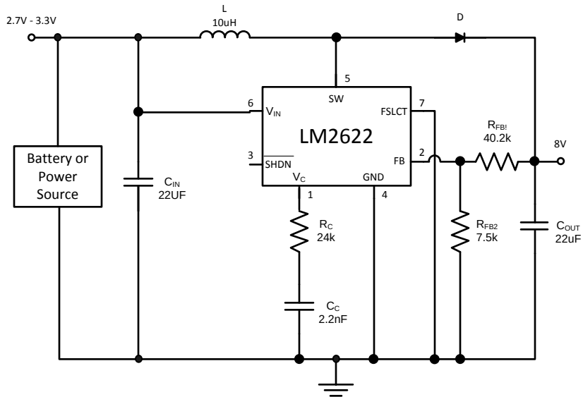
Figure 20. 600 kHz operation
