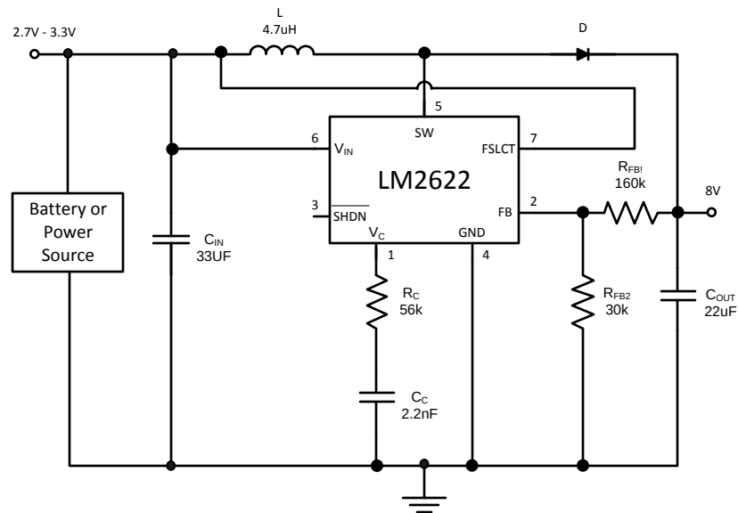
Figure 21. 1.3 MHz operation
