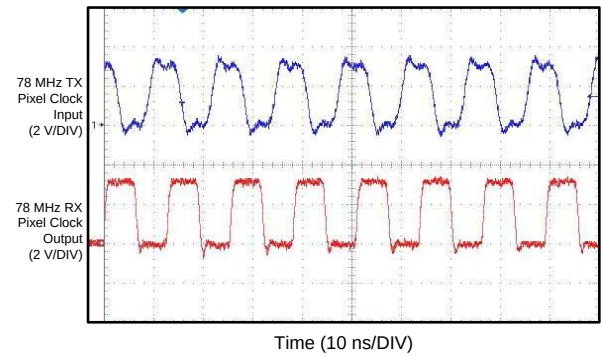
Figure 10. Comparison of Deserializer LVCMOS RX PCLK Output Locked to a 78 MHz TX PCLK
