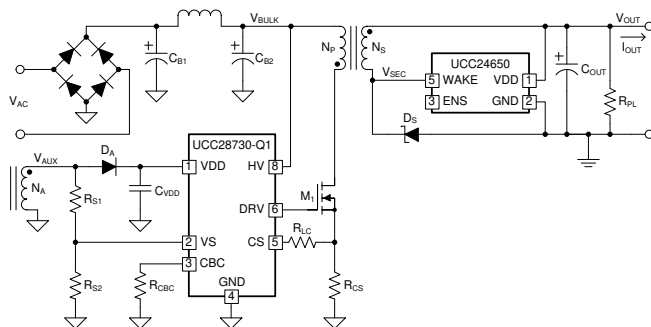
Simplified Schematic
