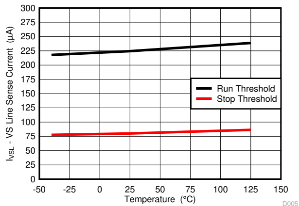
Figure 6-5. VS Line-Sense Current vs. Temperature
