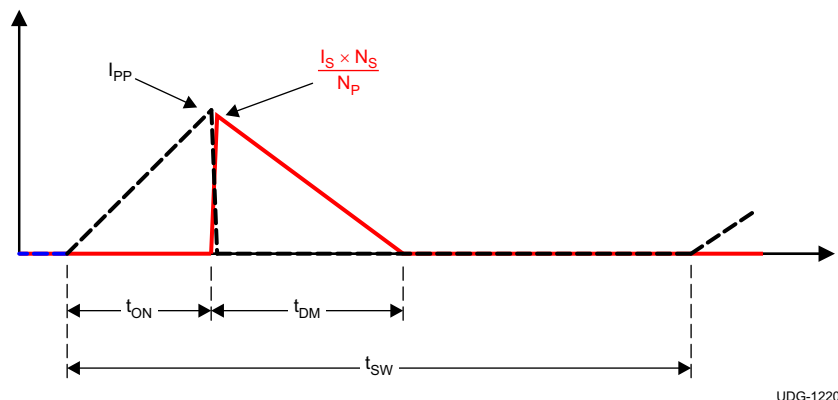
Figure 7-5. Transformer Currents Relationship
