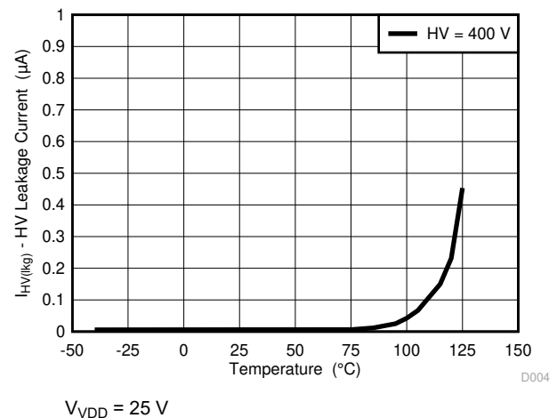
Figure 6-4. HV Leakage Current vs. Temperature
