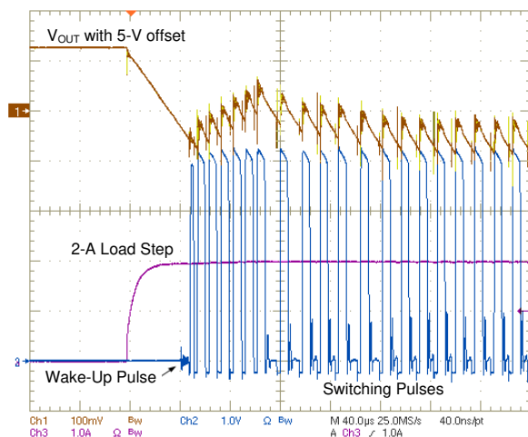
Figure 8-4. Wake-Up Pulse Triggering Response from UCC28730-Q1 Primary-Side Controller
