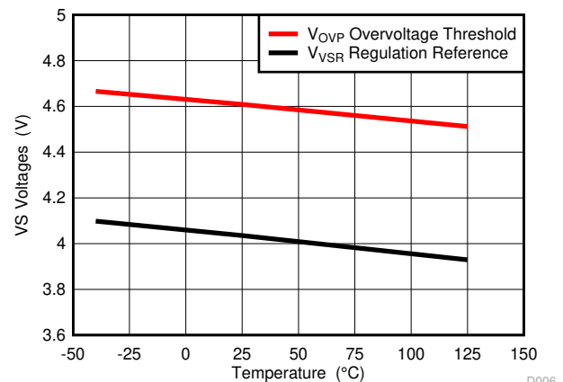
Figure 6-6. VS Voltages vs. Temperature
