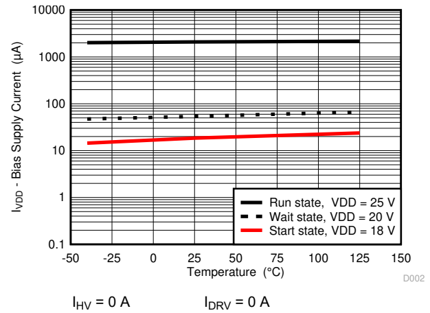
Figure 6-2. Bias Supply Current vs. Temperature
