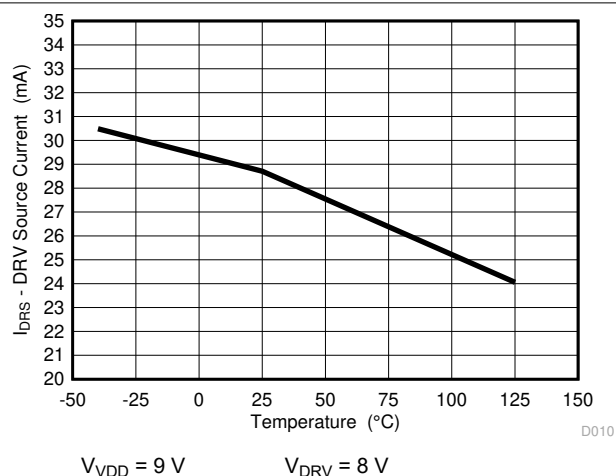
Figure 6-10. DRV Source Current vs. Temperature
