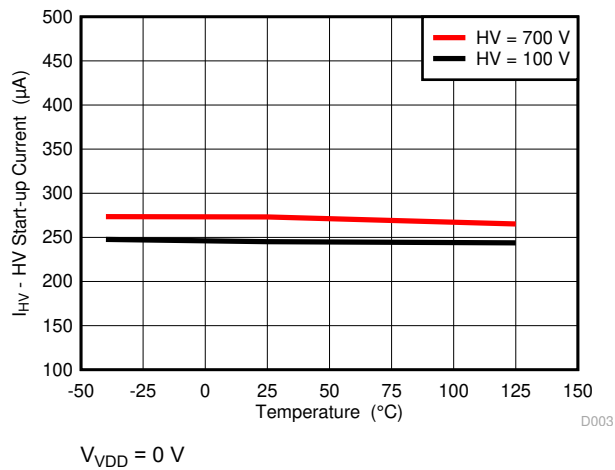
Figure 6-3. HV Start-up Current vs. Temperature
