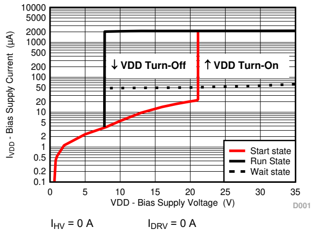
Figure 6-1. Bias Supply Current vs. Bias Supply Voltage
