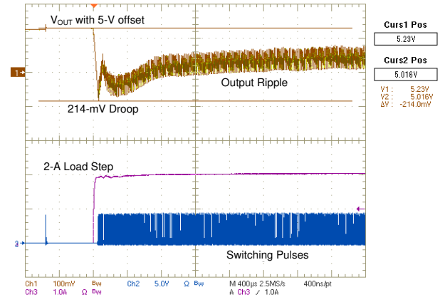
Figure 8-3. Transient Response Detail for 2-A Load Step
