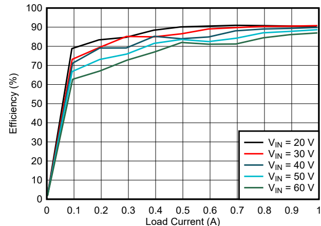
Typical Efficiency, V OUT = 16.4 V
