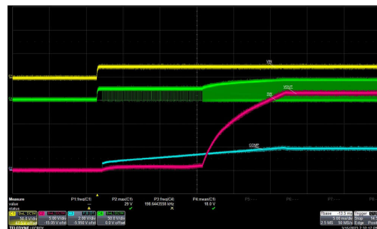
Figure 8-5. Start-Up Characteristic at Full Load
