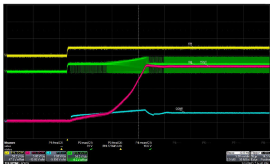
Figure 8-4. Start-Up Characteristic at No Load
