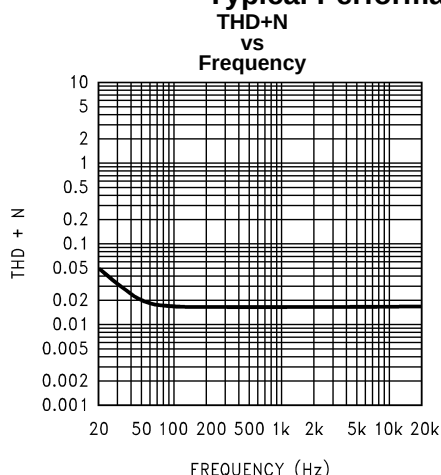
Figure 16. V_{DD} = 5V ; LINEOUT; V_O = 1V_{RMS} ; R_L = 5k\Omega ; Mode 10; 0dB Gain
