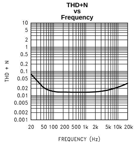
Figure 15. V_{DD} = 3V ; LINEOUT; V_O = 1V_{RMS} ; R_L = 5k\Omega ; Mode 5; 0dB Gain
