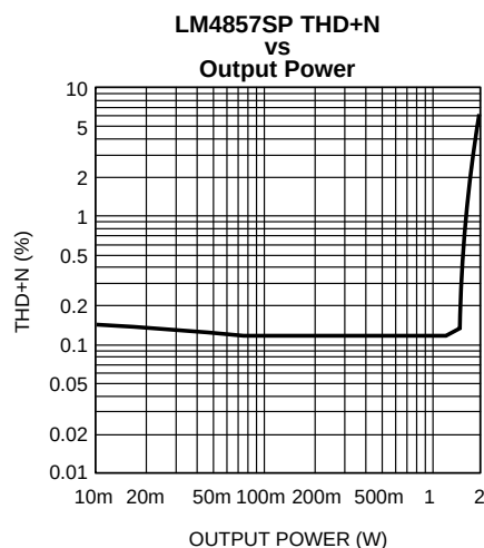
Figure 6. V_{DD} = 5V ; LLS, RLS; f = 1kHz ; R_L = 4\Omega ; Mode 7; 0dB Gain
