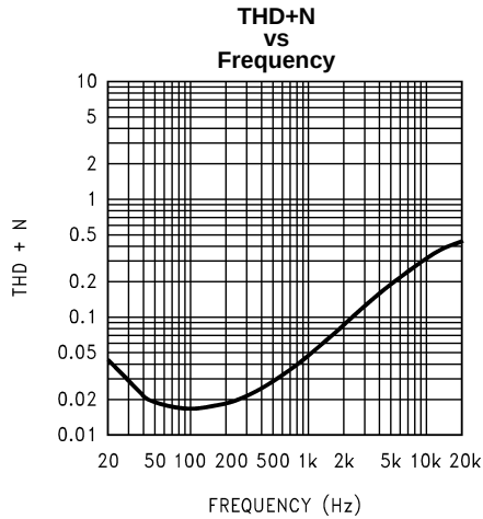
Figure 12. V_{DD} = 5V ; EP; P_O = 15mW ; R_L = 32\Omega ; Mode 1; 0dB Gain, CD4 = 0
