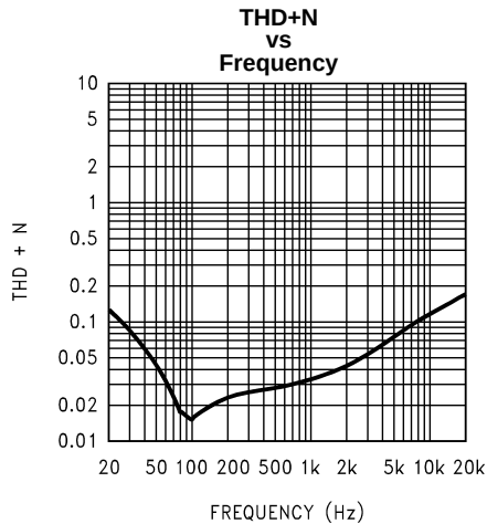
Figure 10. V_{DD} = 5V ; LHP, RHP; P_O = 15mW ; R_L = 32\Omega ; Mode 9; 0dB Gain
