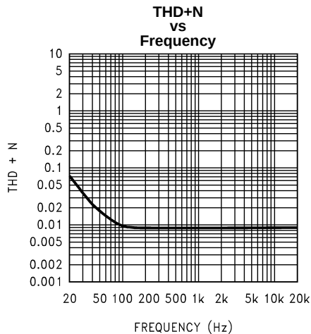
Figure 14. V_{DD} = 5V ; LINEOUT; V_O = 1V_{RMS} ; R_L = 5k\Omega ; Mode 5; 0dB Gain
