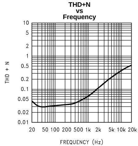
Figure 13. V_{DD} = 3V ; EP; P_O = 10mW ; R_L = 32\Omega ; Mode 1; 0dB Gain, CD4 = 0
