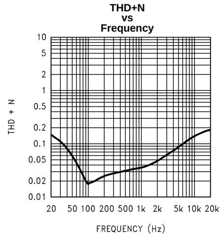
Figure 11. V_{DD} = 3V ; LHP, RHP; P_O = 10mW ; R_L = 32\Omega ; Mode 9; 0dB Gain
