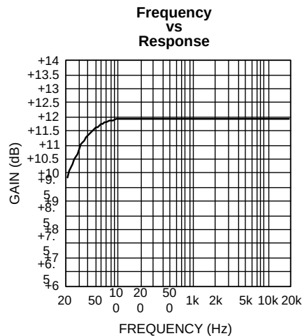
Figure 37. LLS, RLS; R_L = 8\Omega ; Mode 7; Full Gain
