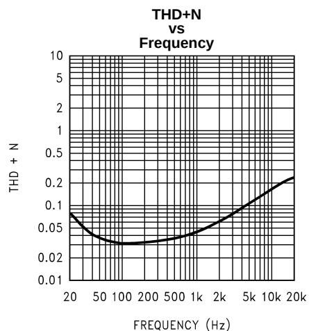
Figure 8. V_{DD} = 5V ; LLS, RLS; P_O = 400mW ; R_L = 8\Omega ; Mode 7; 0dB Gain
