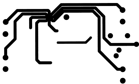
Figure 50. Recommended SOIC PC Board Layout: Bottom Layer
