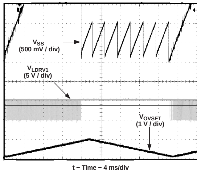
Figure 26. Overvoltage, Latch and Re-Start
