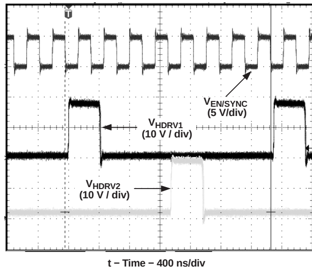
Figure 24. External Clock on EN/SYNC
