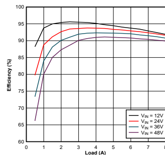
Typical Efficiency V_{\text{OUT}} = 5\text{V} , f_{\text{SW}} = 400\text{kHz}
