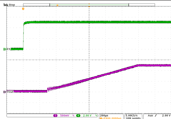
Figure 10-52. Start-Up Timing
