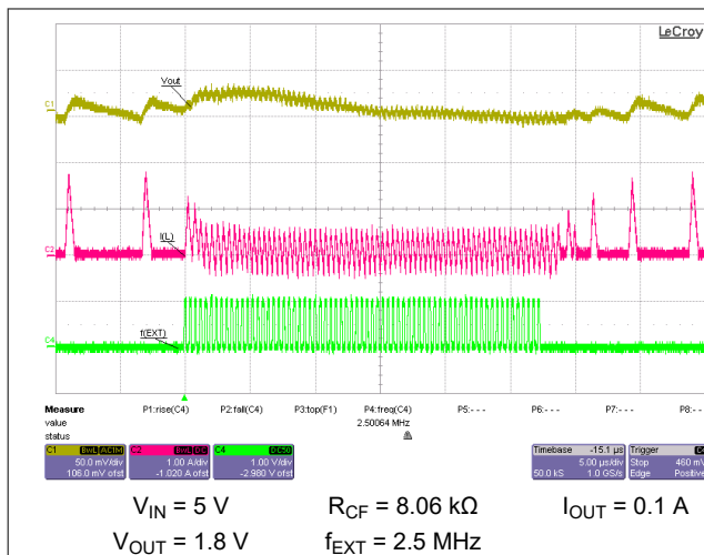
Figure 10-61. Switching from External Synchronization to Power-Save Mode (PFM)
