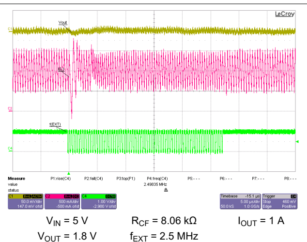
Figure 10-62. Switching from External Synchronization to Internal Fixed Frequency
