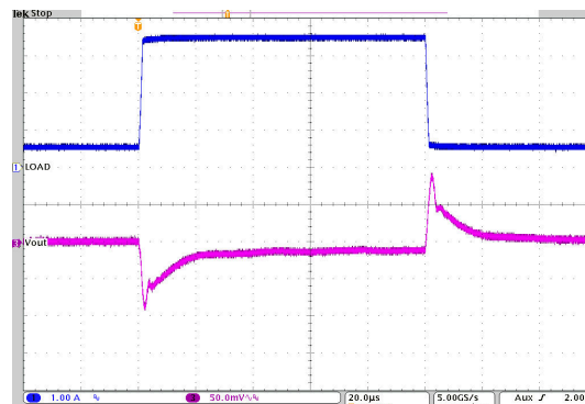
Figure 10-27. Load Transient Response
