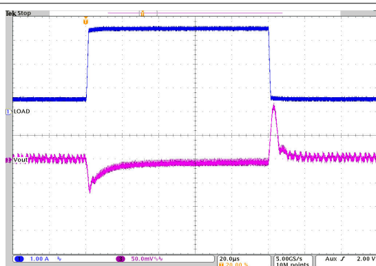
Figure 10-26. Load Transient Response
