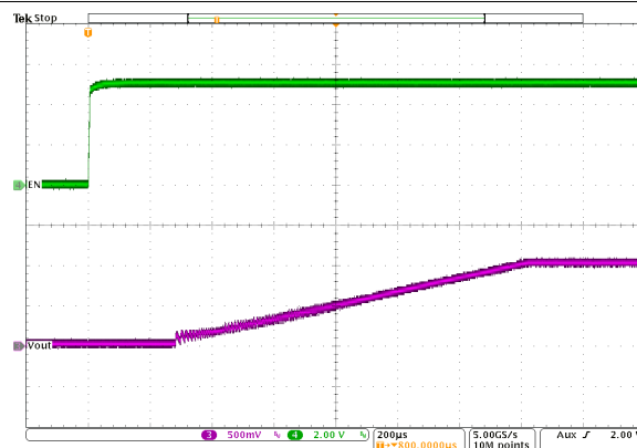
Figure 10-53. Start-Up Timing
