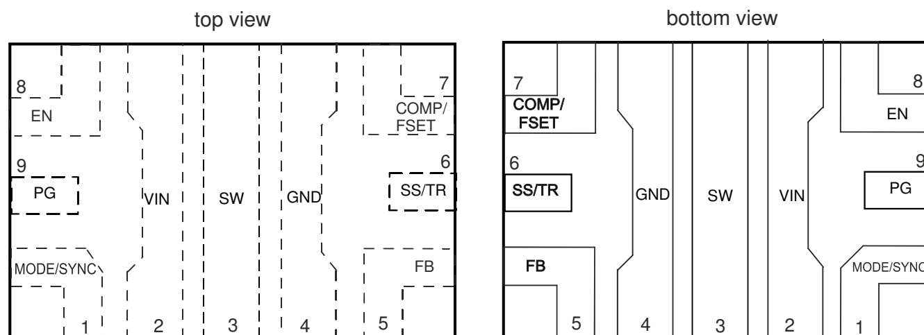
Figure 6-1. RWY Package 9 Pin (VQFN)
