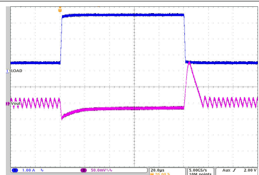
Figure 10-28. Load Transient Response
