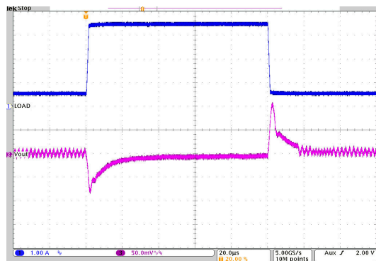
Figure 10-26. Load Transient Response
