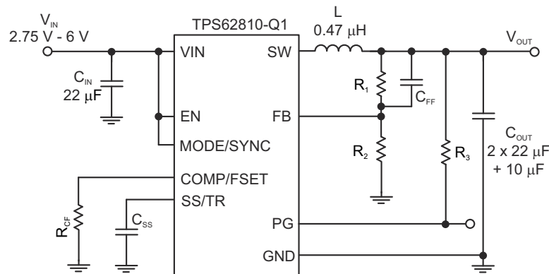
Figure 10-1. Typical Application
