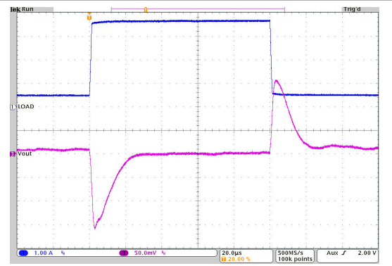
Figure 10-21. Output Voltage versus Output Current
