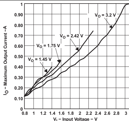
Figure 5. Maximum Output Current vs Input Voltage
