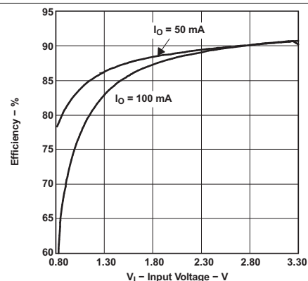
Figure 4. Efficiency vs Input Voltage
