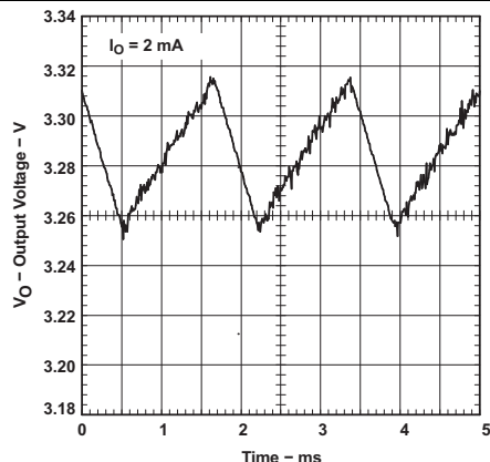
Figure 19. TPS61006 Output Voltage Ripple Amplitude
