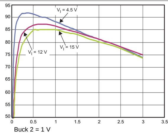
Figure 4. Efficiency
