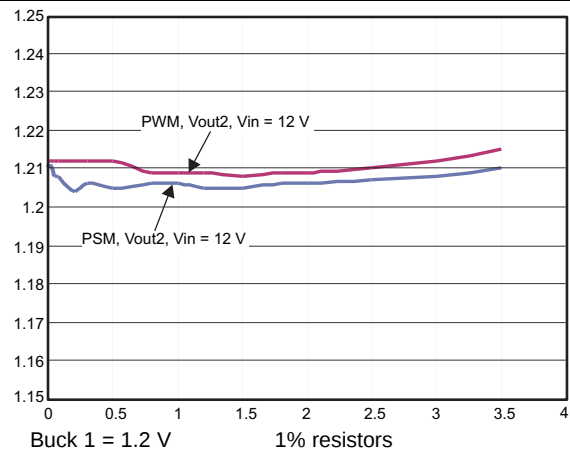
Figure 2. Load Regulation
