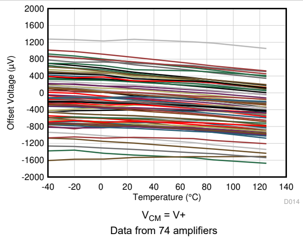
Figure 5-4. Offset Voltage vs Temperature
