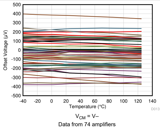
Figure 5-3. Offset Voltage vs Temperature
