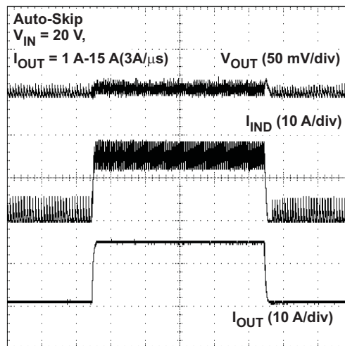
0.9-V LOAD TRANSIENT RESPONSE
