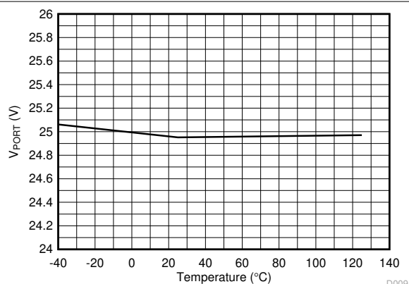
Figure 7-9. Discovery Open Circuit Voltage vs Temperature
