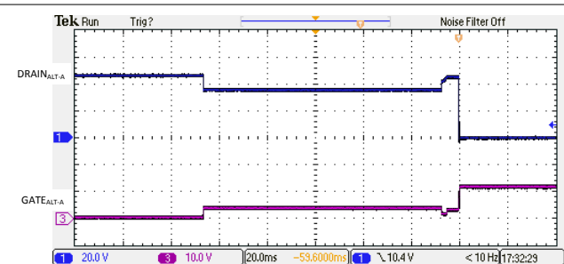
Figure 10-15. 2-Pair 1-Finger Classification and Turn On
