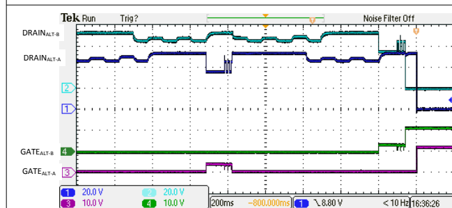
Figure 10-18. 4-Pair Single Signature Discovery and Turn On from Semi-Auto Mode
