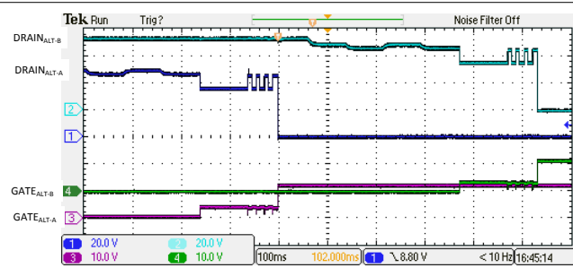
Figure 10-27. 4-Pair Dual Signature 4-Finger Classification and Turn On
