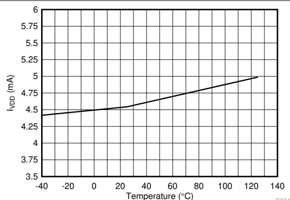
Figure 7-4. VDD Current Consumption vs Temperature
