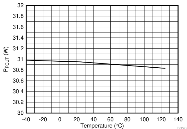
Figure 7-20. 2-Pair PCut Threshold (30W) vs Temperature
