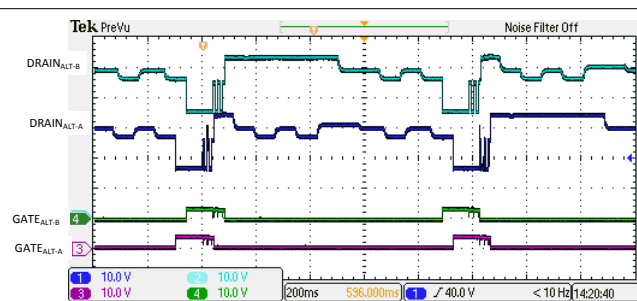
Figure 10-23. 4-Pair Semi-Auto Mode Discovery with a Valid Dual Signature Class 4D Load
