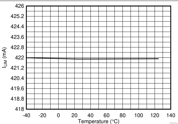
Figure 7-24. 1x Mode (2xFBn = 0) Current Limit vs Temperature
