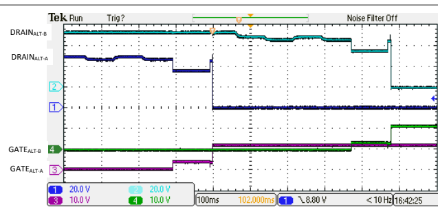
Figure 10-25. 4-Pair Dual Signature 1-Finger Classification and Turn On
