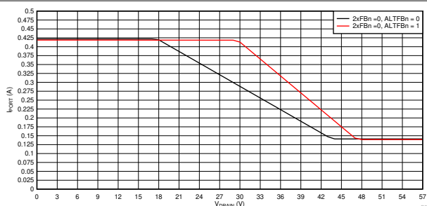
Figure 9-55. 1x Mode (2xFBn = 0) Foldback Curves, I_{PORT} vs V_{DRAIN}
