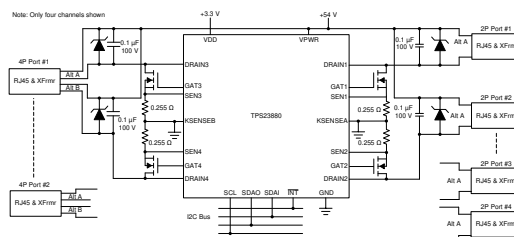
Simplified Schematic
