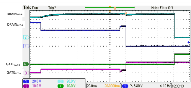
Figure 10-19. 4-Pair Single Signature 1-Finger Classification and Turn On
