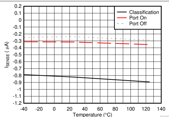
Figure 7-6. SENSE Pin Bias Current vs Temperature
