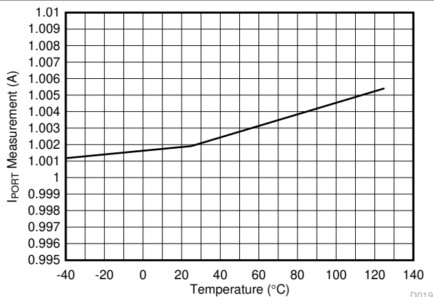
Figure 7-19. Port Current ADC Measurement (1 A) vs Temperature
