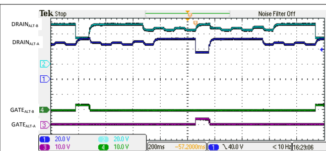
Figure 10-17. 4-Pair Semi-Auto Mode Discovery with a Valid Single Signature Class 0-3 Load
