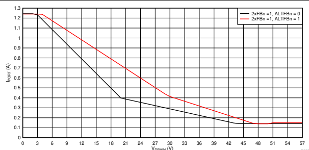
Figure 9-56. 2x Mode (2xFBn = 1) Foldback Curves, I_{PORT} vs V_{DRAIN}
