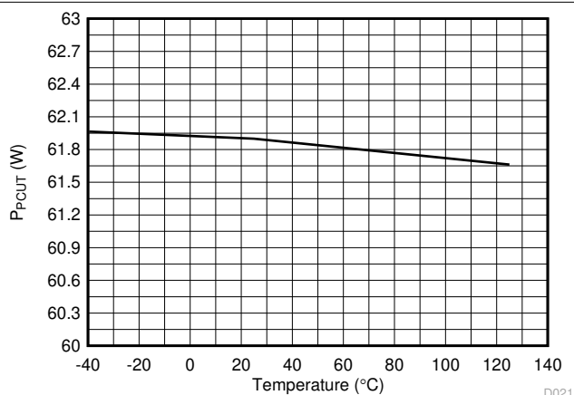
Figure 7-21. 4-Pair PCut Threshold (60W) vs Temperature
