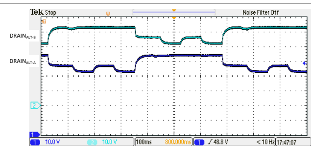
Figure 10-13. 4-Pair High Resistance (36kΩ) Detection Signature
