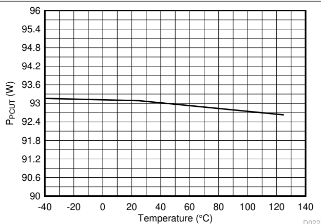
Figure 7-22. 4-Pair PCut Threshold (90W) vs Temperature
