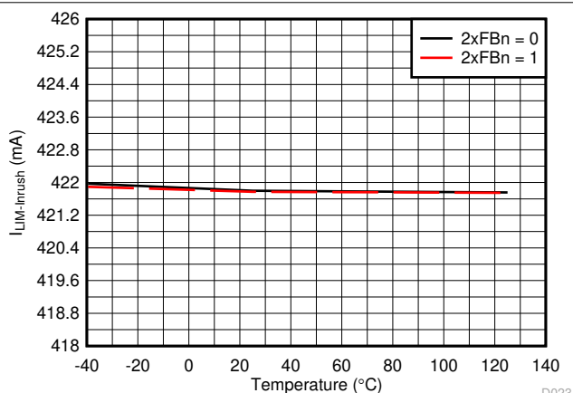
Figure 7-23. Inrush Current Limit vs Temperature
