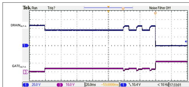
Figure 10-16. 2-Pair 3-Finger Classification and Turn On
