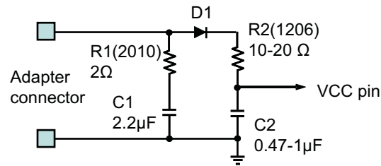
Figure 9. Input Filter
